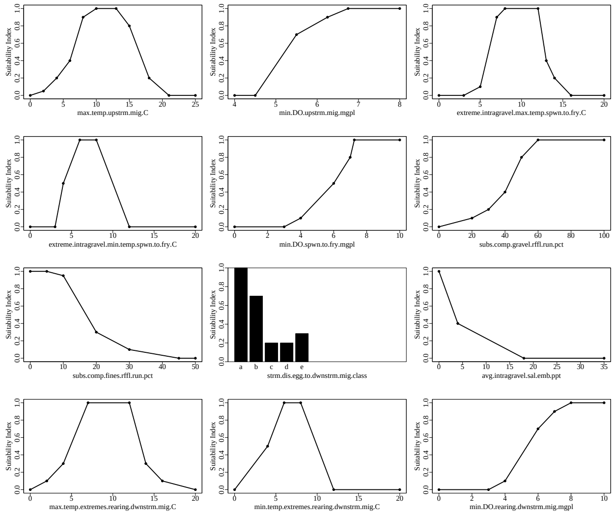
Figure 1. Suitability index graphs for variables included in the chumsalmonEyedEmb model in ecorest.
