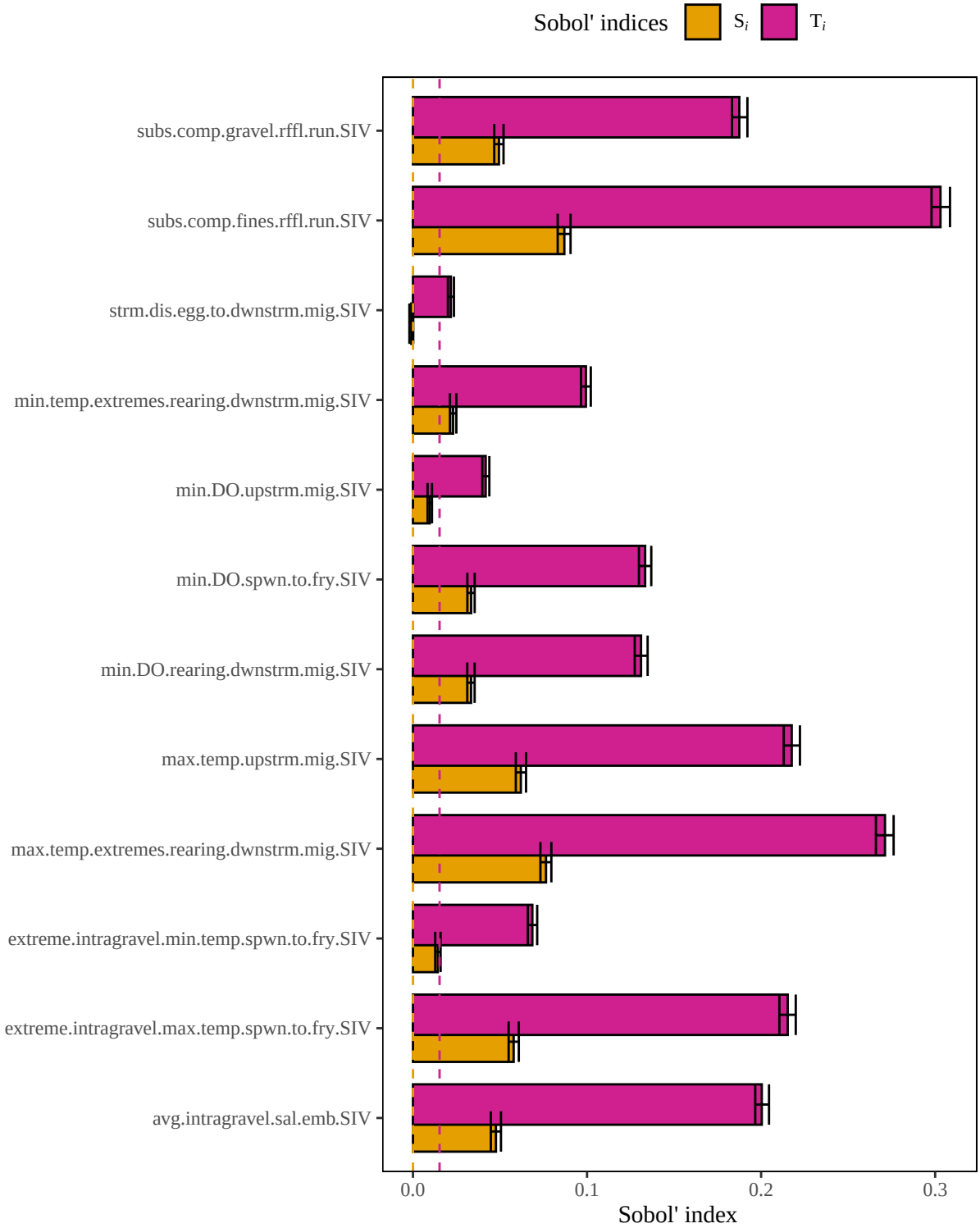
Figure 6. Results of a sensitivity analysis for the chumsalmonEyedEmb model based on a limiting factor structure. Dashed lines represent baseline numerical approximation error for S_i and T_i ( i.e. , dummy variables).
