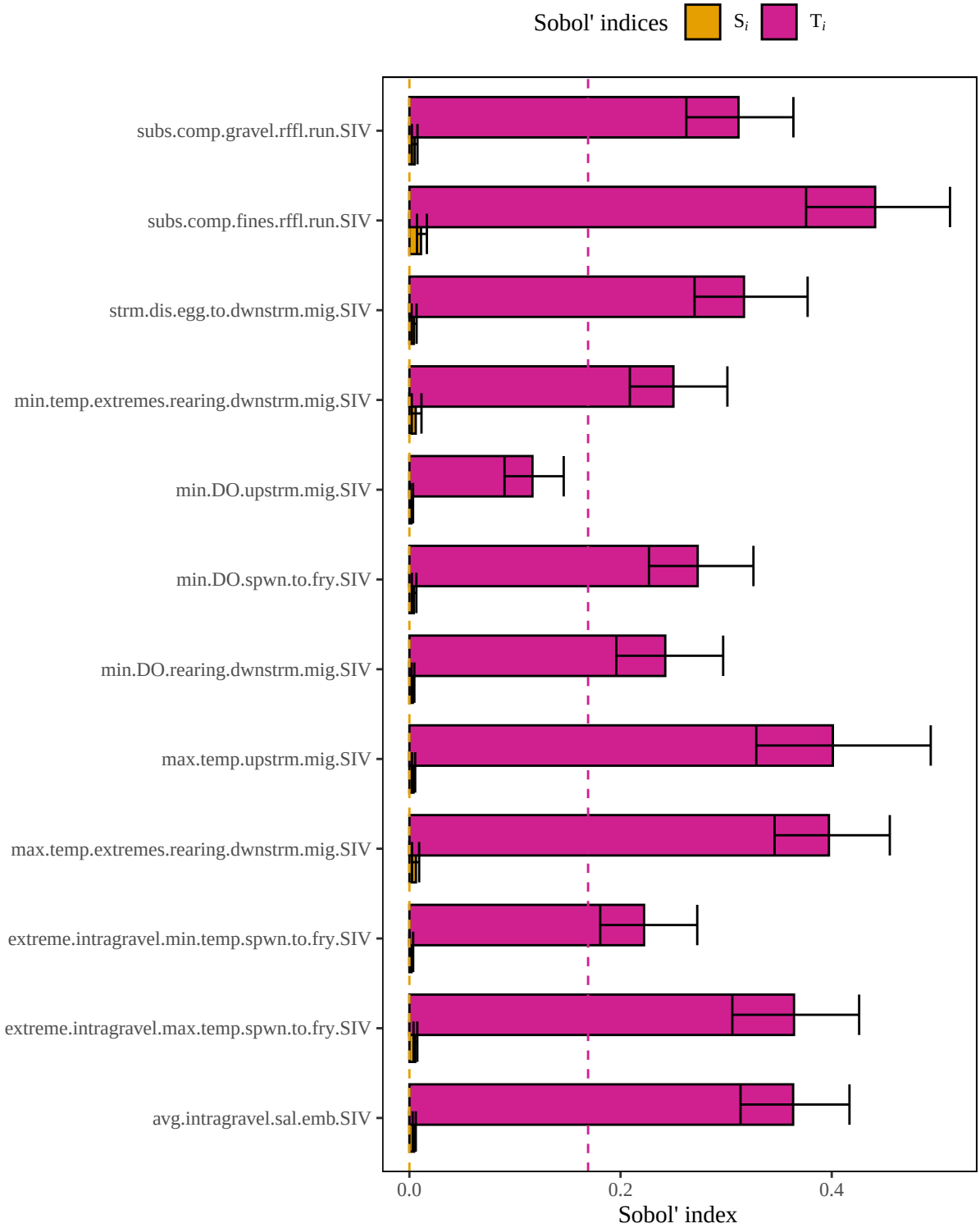
Figure 7. Results of a sensitivity analysis for the chumsalmonEyedEmb model based on a multiplicative mean structure. Dashed lines represent baseline numerical approximation error for S_i and T_i ( i.e. , dummy variables).
