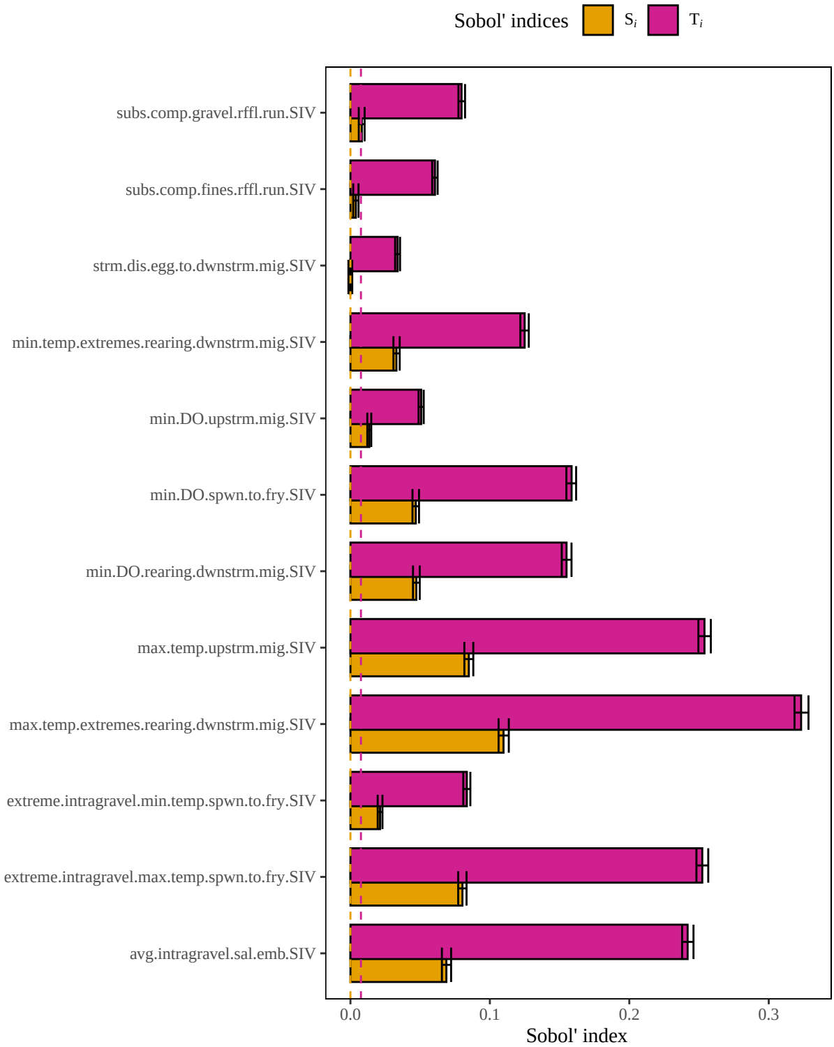
Figure 3. Results of a sensitivity analysis for the chumsalmonEyedEmb model based on the original limiting factor model outlined in Hale et al. (1985). Dashed lines represent baseline numerical approximation error for S_i and T_i ( i.e. , dummy variables).
